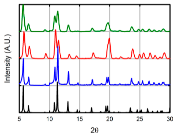
Figure 3. Powder X-ray diffractograms of simulated UiO-67 (black), UiO-67 (blue), UiO-67-Squar/bpdc (red), and post-catalysis UiO-67-Squar/bpdc (green). Peaks at 2\theta > 10 have been enhanced by 10 \times for clarity. The PXRD patterns of the urea-containing derivatives have been reported elsewhere. 45
